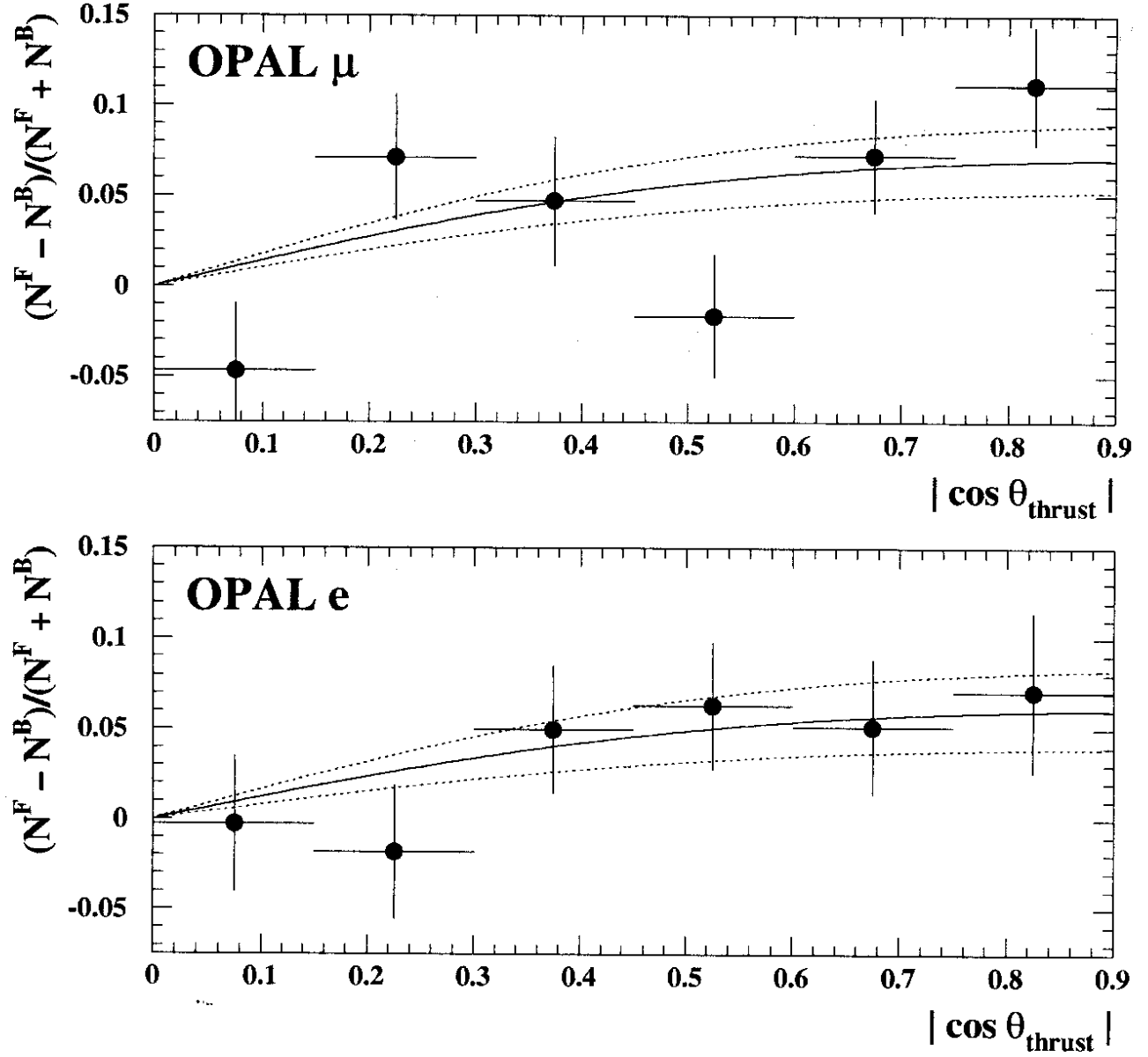
Figure 9: The ratio (N^F - N^B)/(N^F + N^B) vs. |y| = |\cos \theta_{\text{thrust}}| , for prompt muons with p > 3 \text{ GeV}/c and p_t > 1 \text{ GeV}/c , and prompt electrons with p > 2 \text{ GeV}/c and p_t > 0.8 \text{ GeV}/c . The curves are of the form 8A_{FB}^{\text{obs}}|y|/3(1+y^2) . The solid curves are for the fitted values of A_{FB}^{\text{obs}} , and the dotted curves are for values of A_{FB}^{\text{obs}} one standard deviation from the fitted values.
