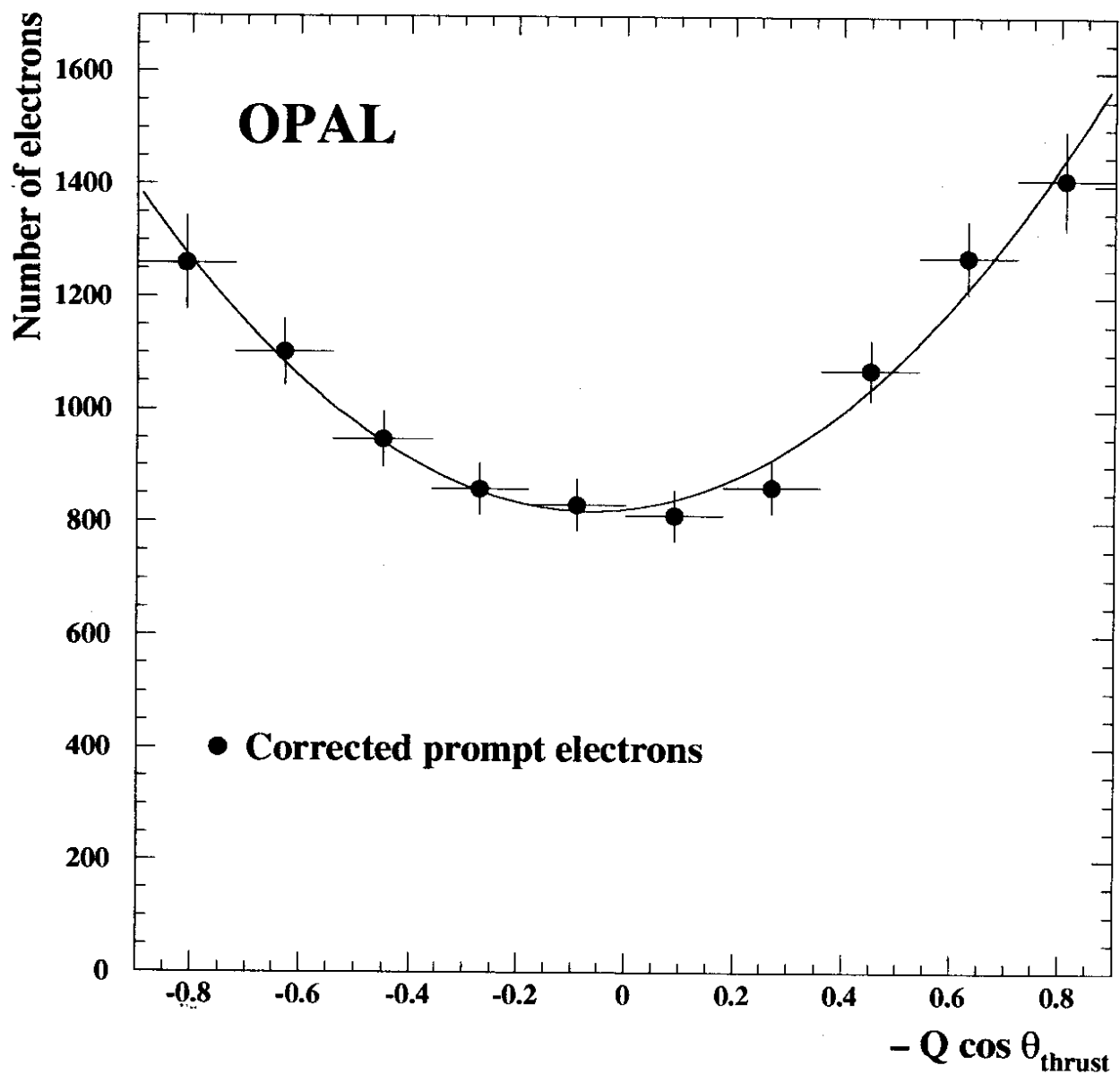
Figure 7: The distribution of y = -Q \cos \theta_{\text{thrust}} for electron candidates with p > 2 \text{ GeV}/c and p_t > 0.8 \text{ GeV}/c , after subtracting non-prompt backgrounds, and correcting for efficiency. The result of an event-by-event likelihood fit to the uncorrected data to measure the effective asymmetry is superimposed.
