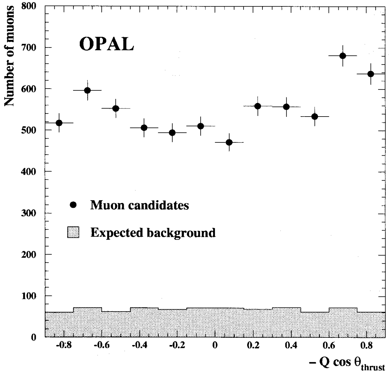
Figure 4: The distribution of y = -Q \cos \theta_{\text{thrust}} for all muon candidates with p > 3 \text{ GeV}/c and p_t > 1 \text{ GeV}/c . The shaded area indicates the predicted hadronic background.
