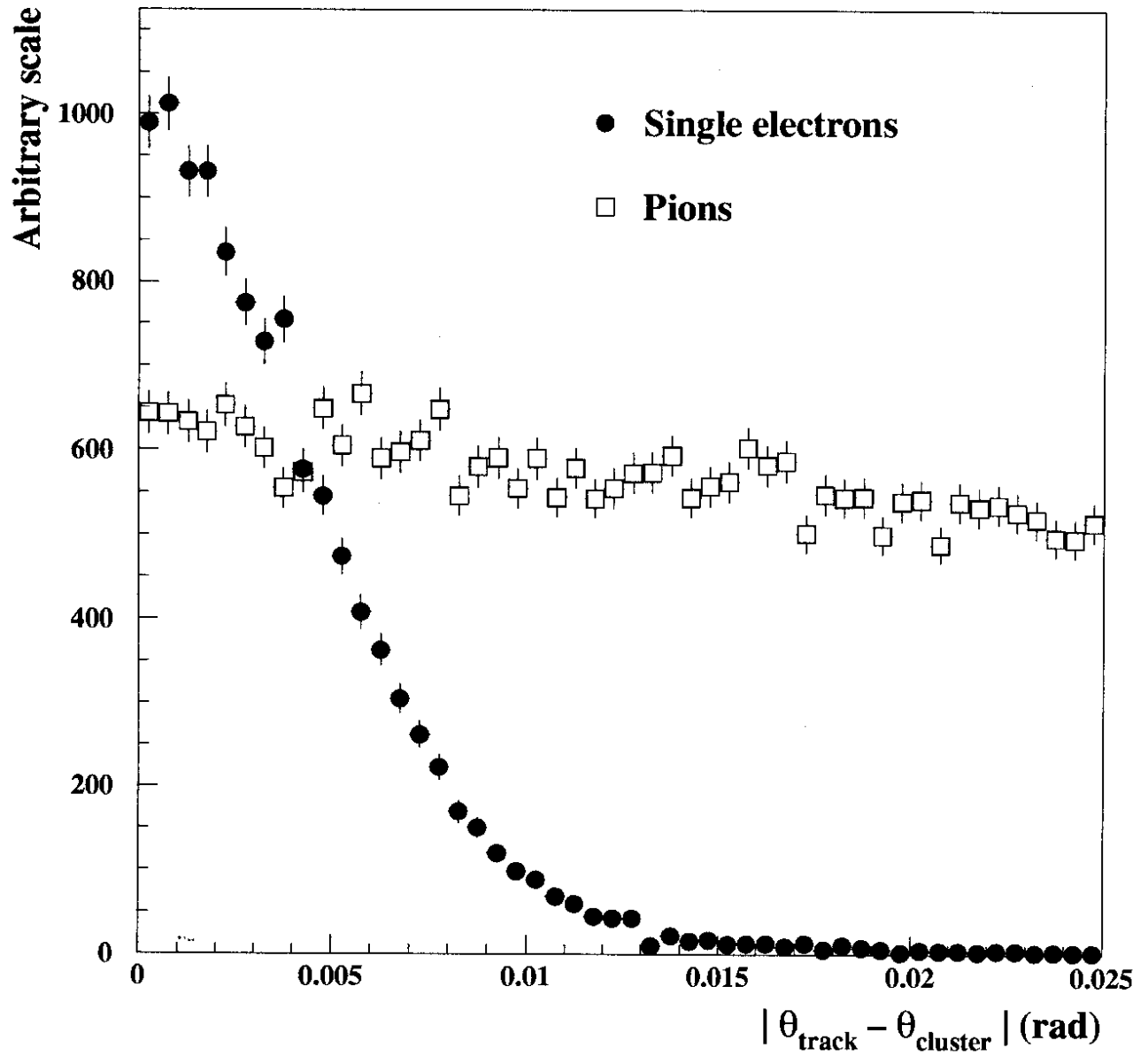
Figure 1: The distribution of |\theta_{\text{track}} - \theta_{\text{cluster}}| for electrons in low multiplicity events and pions from K^0 decays. The electron selection cut is at 8 mrad.
