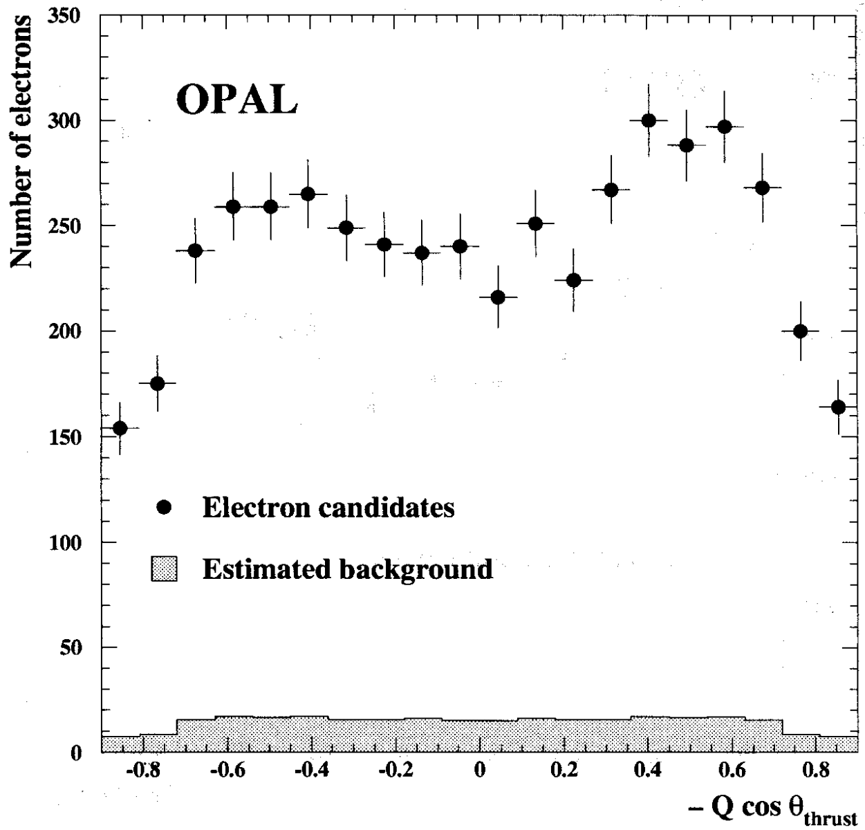
Figure 6: The distribution of y = -Q \cos \theta_{\text{thrust}} for all electron candidates with p > 2 \text{ GeV}/c and p_t > 0.8 \text{ GeV}/c .
