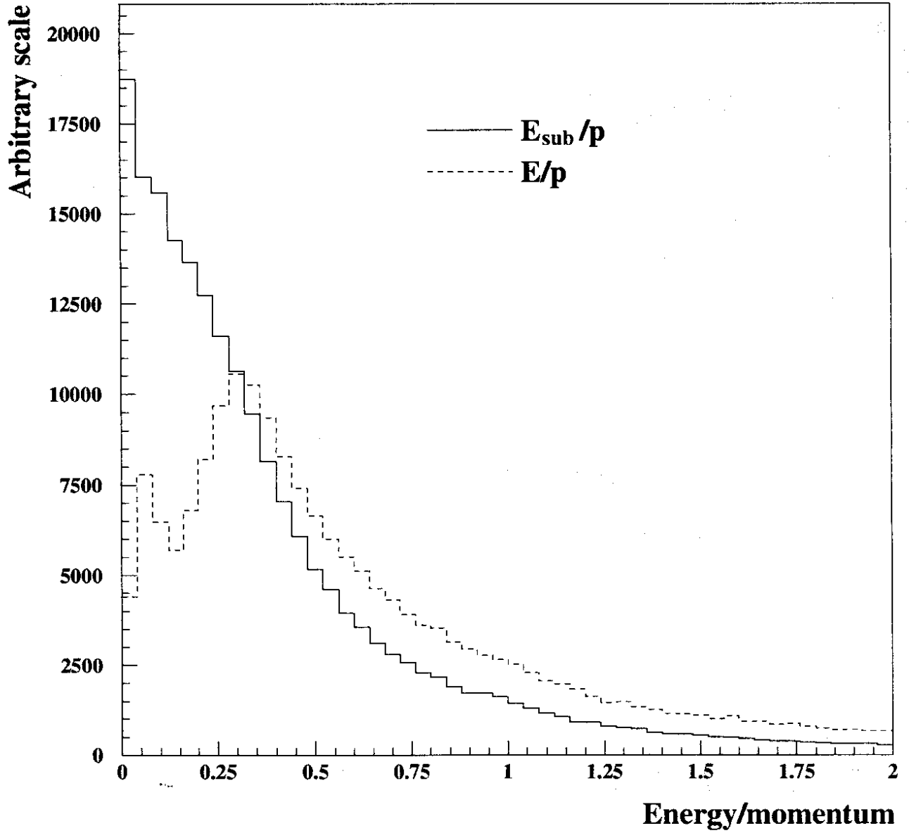
Figure 3: The background subtracted energy-momentum ratio, E_{\text{sub}}/p , compared to the ratio of the cluster energy to momentum, E/p , for pions from K^0 decays. In the signal region ( 0.8 < E_{\text{sub}}/p < 1.2 ), the modified energy estimate provides a reduced background.
